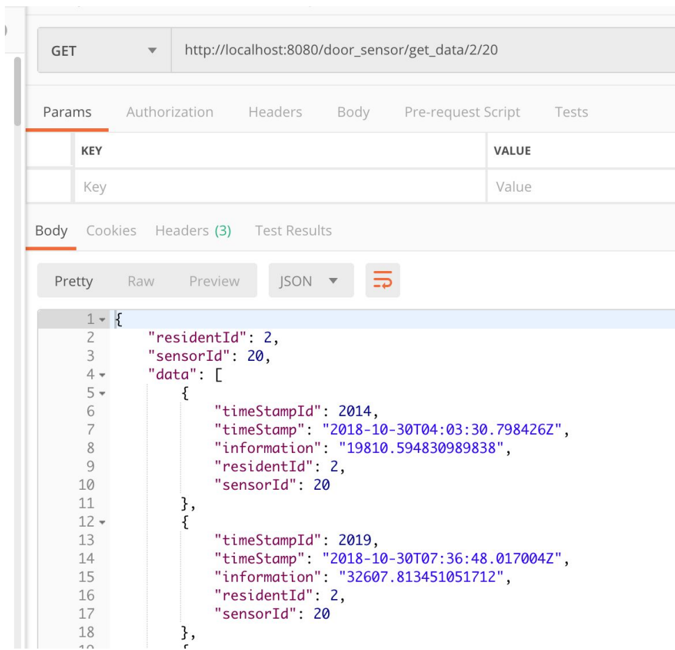
Figure: 3.6.5: The response from our server.(Search data by specific sensor_id and resident_id)
